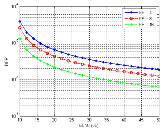
Figure 7. BER vs E_b/N_0 by varying size of spreading factors.
