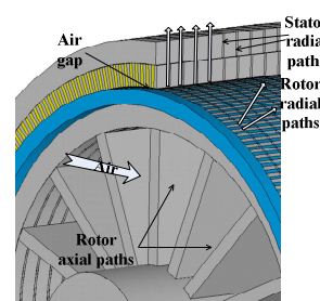
Figure 6. Air-flow near iron core in the new structure
