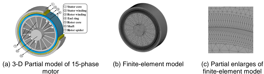
Figure 2. the 3-D calculation model
