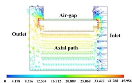
Figure 4. Cross-sectional view of air velocity distribution. The air-flow speed is indicated by arrow field
