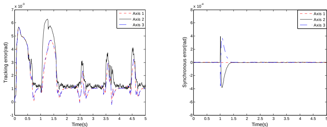
Figure 6. Tracking Error and Synchronous Error of each Shaft when there's Load Disturbance on Single Shaft
