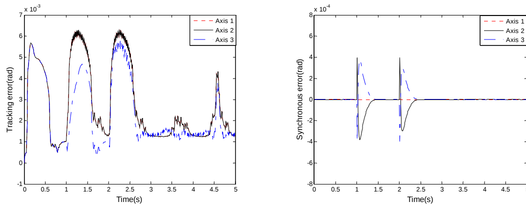
Figure 7. Tracking Error and Synchronous Error when there're Load Disturbances on Multi-shaft
