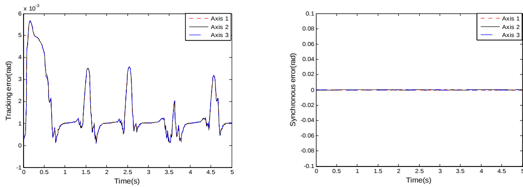
Figure 5. Multi-shaft Tracking Error and Synchronous Error when there's no External Load Disturbance
