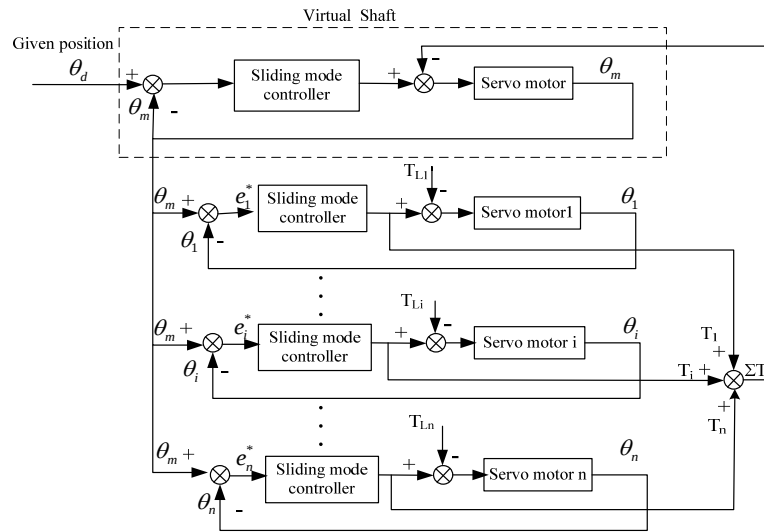
Figure 3. Structure Diagram of Electronic Virtual Line Shifting Control-Based Multi-shaft Coordinating Control System
