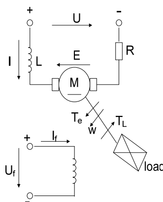
Figure 1. DC Motor Circuit and Mechanical Connection Schematic
