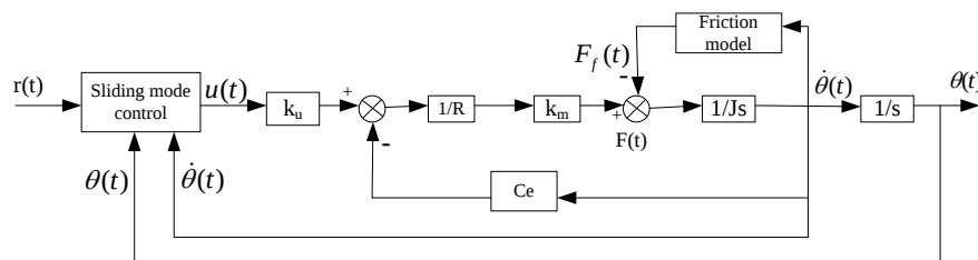
Figure 2. Control Structure Diagram of Single Shaft System
