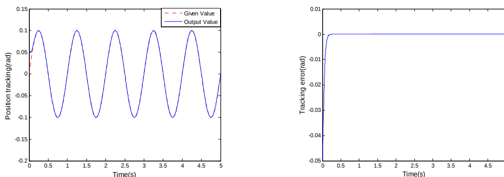
Figure 4. Single-shaft Position Tracking and Tracking Error when there's no External Load Disturbance
