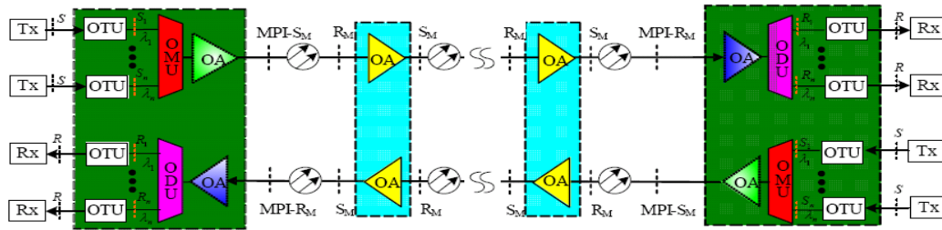
Figure 4. The Reference Configuration of 40G DWDM System
