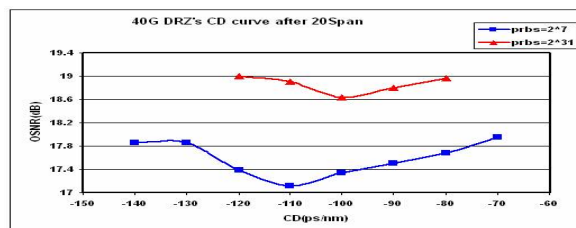
Figure 11. 40G DWDM Transmission 1600km System Dispersion Curve
