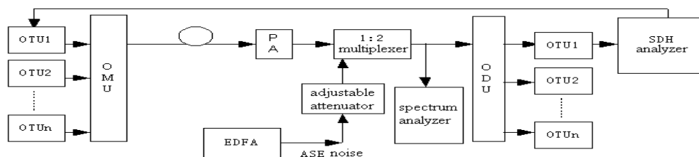
Figure 6. Configuration diagram of 40 G OTU OSNR Performance Test
