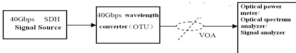
Figure 5. Configuration Diagram of 40 G OTU Performance Test
