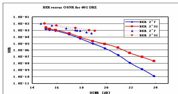
Figure 9. 40G DWDM System back-to-back Testing of BER and OSNR Based on DRZ
