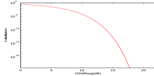
Figure 3. The Relation Curve of BER and OSNR_{avg}
