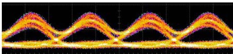
Figure 8. DRZ 40G DWDM OTU Typical Eye Diagram
