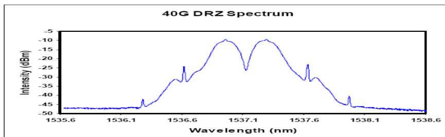
Figure 7. DRZ 40G DWDM OTU Typical Spectrum
