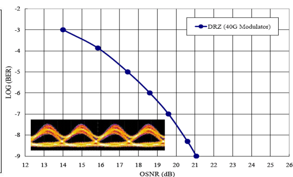
Figure 10. 40G DWDM 1600km long-fiber Transmission BER and OSNR Curve
