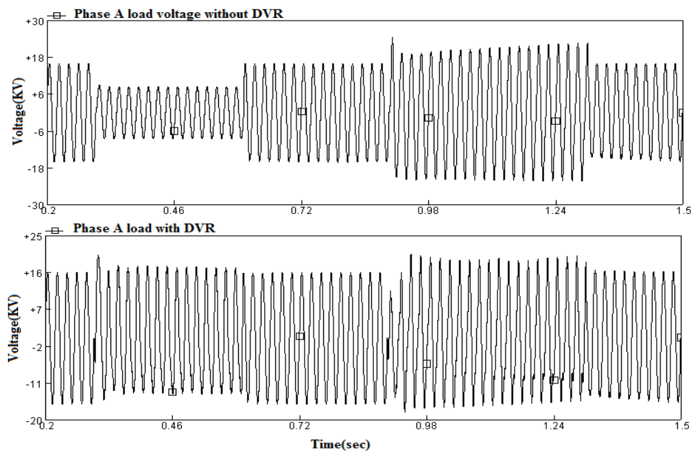
Figure15: Voltage of one of the phases' load (A) with and without DVR
