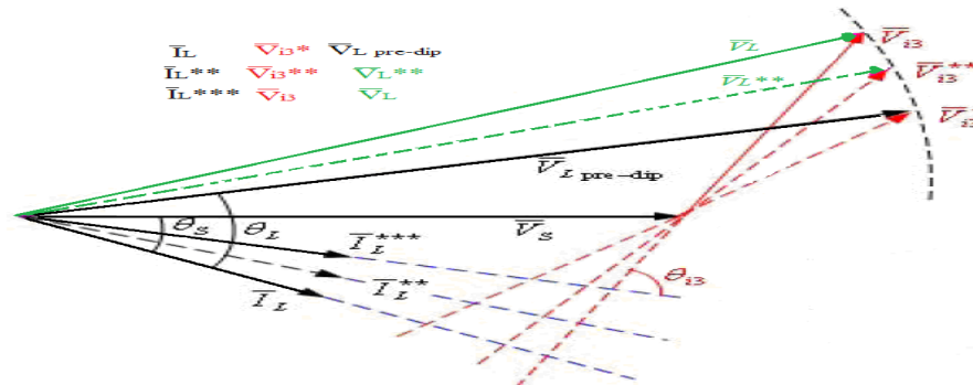
Figure8: phasors diagram of PAC method
