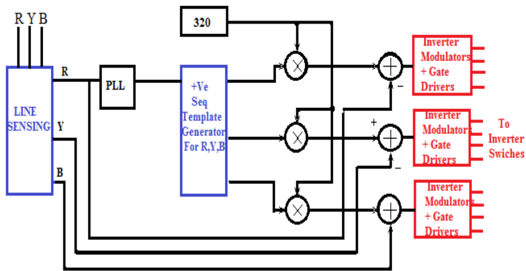
Figure11: Block diagram of Control strategy for a DVR
