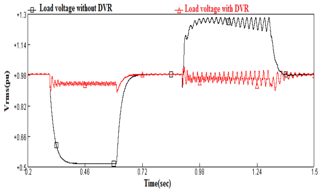
Figure 16: Voltage (pu) of one of the phases' load (A) with and without DVR
