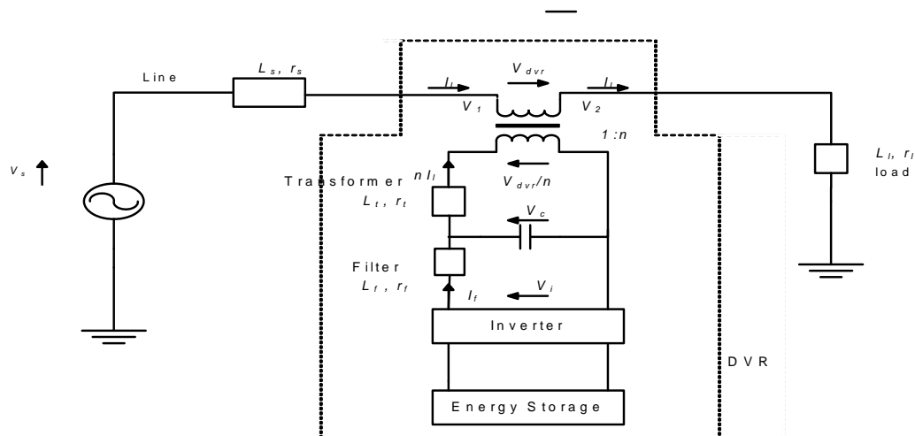
Figure 2 : Distribution system with DVR
