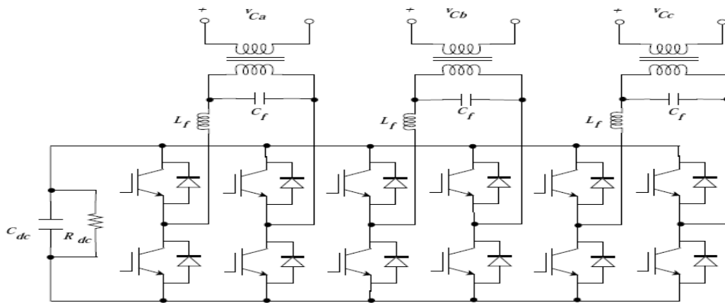
Figure5: Structure and configuration of DVR.
