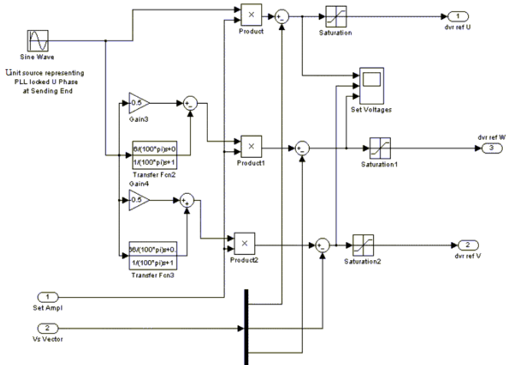
Figure12: Reference block of Inverter
