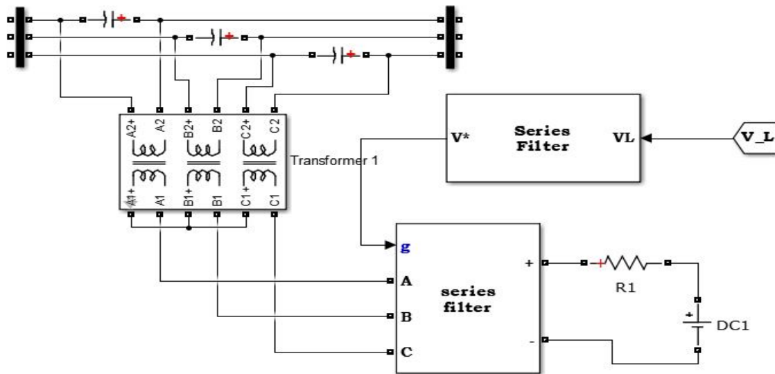
Figure13: Schematics of a simulated DVR and its performance
