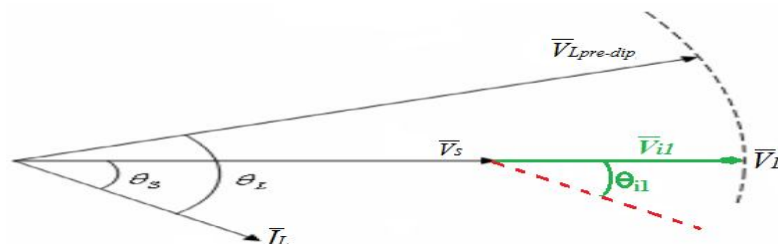
Figure6: Phasors diagram of the IPC method
