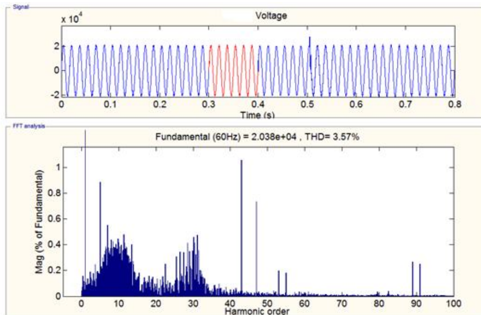
Figure 19: Grid voltage and its harmonic distribution after compensation by DVR
