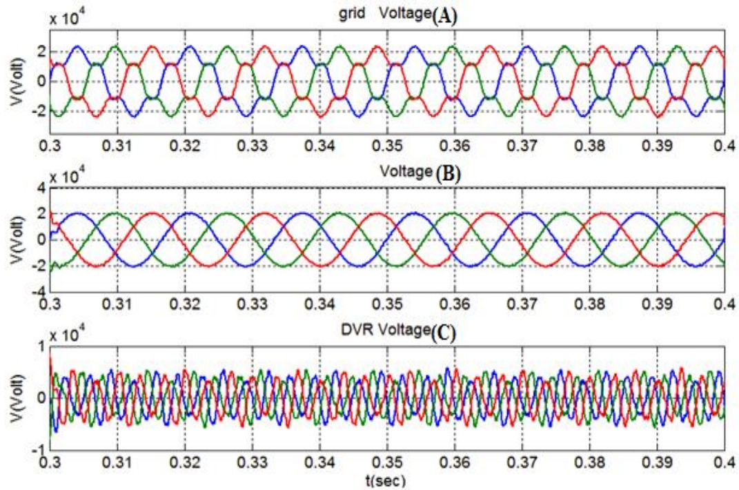
Figure 18: Compensation of voltage harmonics by DVR, grid voltage contains harmonics of 5 th , 7 th (A), compensated voltage by DVR (B) , injected voltage by DVR (C)
