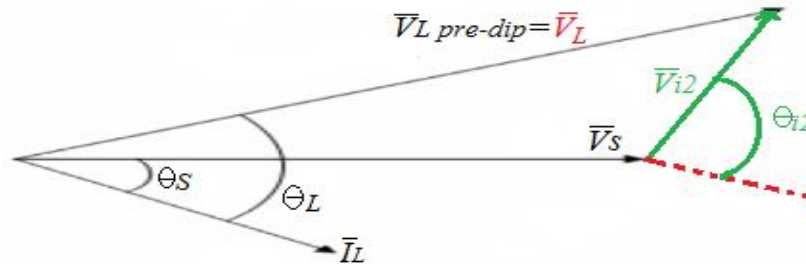
Figure 7: phasors diagram of the PDC method
