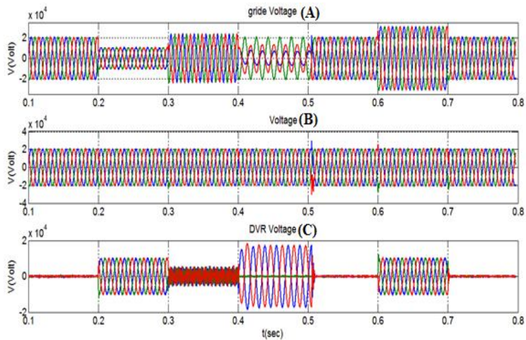
Figure 17: Grid voltage (A) , compensated voltage by DVR (B) , injected voltage by DVR (C)
