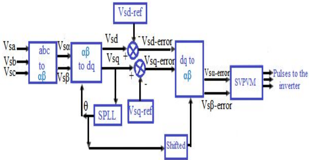
Figure10: Block diagram of control system
