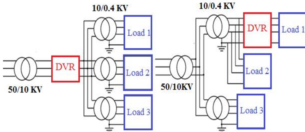
Figure3: Placement of DVR's in distribution networks
