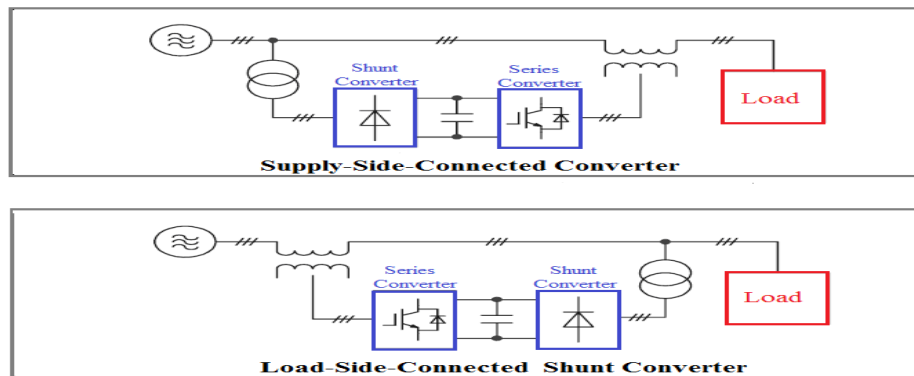
Figure9: Topologies for DVRs without energy storage
