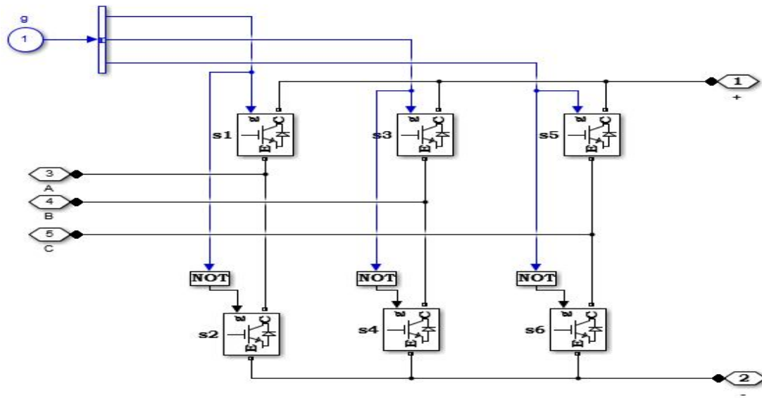
Figure14: Power circuit of DVR
