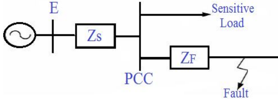
Figure 1 : Voltage divider model for voltage sag
