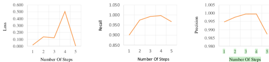
Figure 6. Loss, recall, and precision method II
