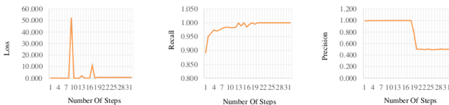
Figure 7. Loss, recall, and precision method III
