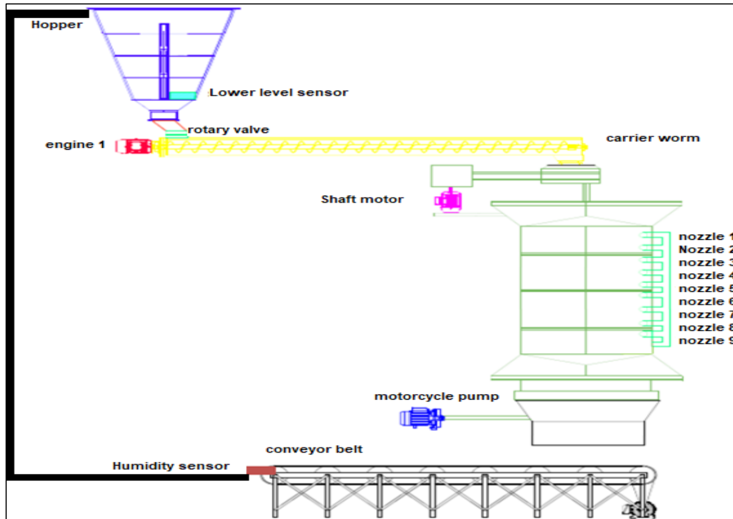
Representation of the industrial process
