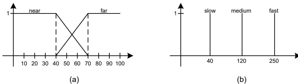
Figure 3. Input MF and output MFvalue (a) Membership Function of distance sensor as input (b) Membership Function of motor speed as output
