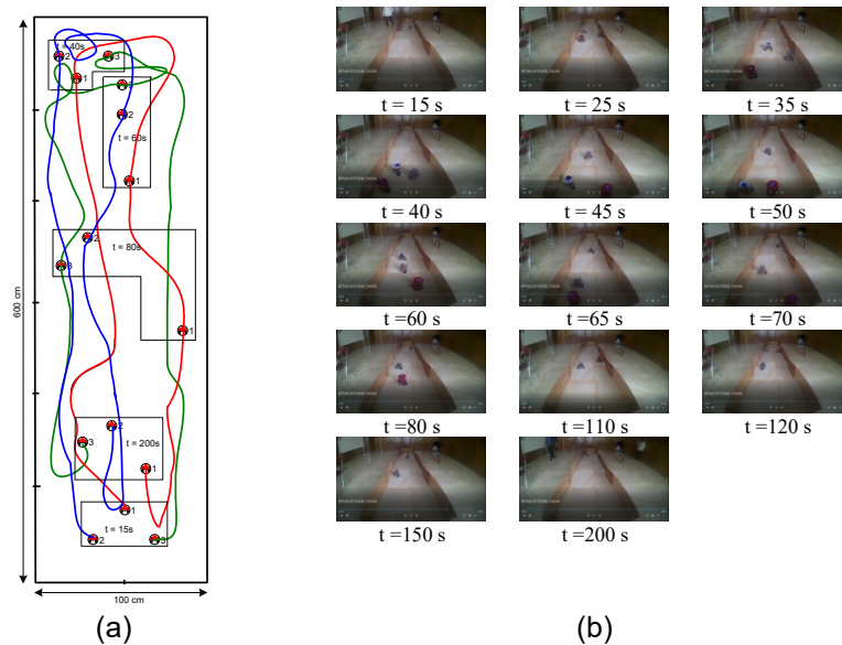
Figure 5. Swarm Robot Coordination Experiments in arena 1x4 m (a) Tracking Robot(b). Experiment Photographs
