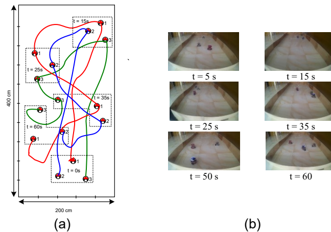
Figure 6. Swarm Robot Coordination Experiments in arena 2x4 m (a) Tracking Robot (b) Experiment Photographs
