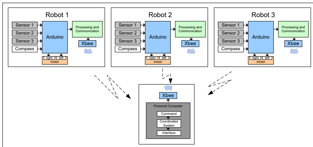
Figure 1. Block diagram control of swarm robot coordination
