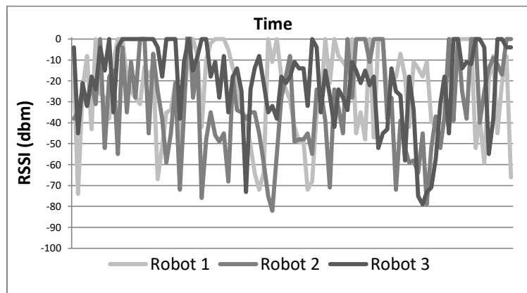
Figure 8. RSSI values from experimental environment
