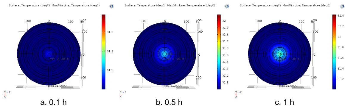
Figure 4. Thermal profiles of a clean insulator surface with 20kV applied voltage for (a) 0.1 of hour, (b) half-hour, and (c) one-hour
