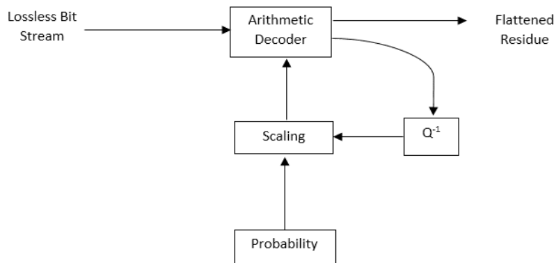
Figure 7. IEEE 1857.2 Entropy Decoder [4]
