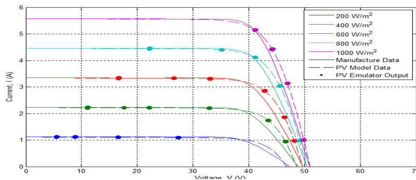
Figure 5. The I-V characteristic curved obtained from the PV model and the manufacturer datasheet compared to the photovoltaic emulator output at 25 °C
