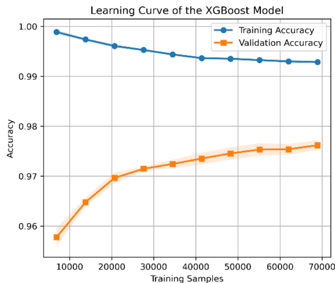
Figure 4. Learning curve of the XGBoost model
