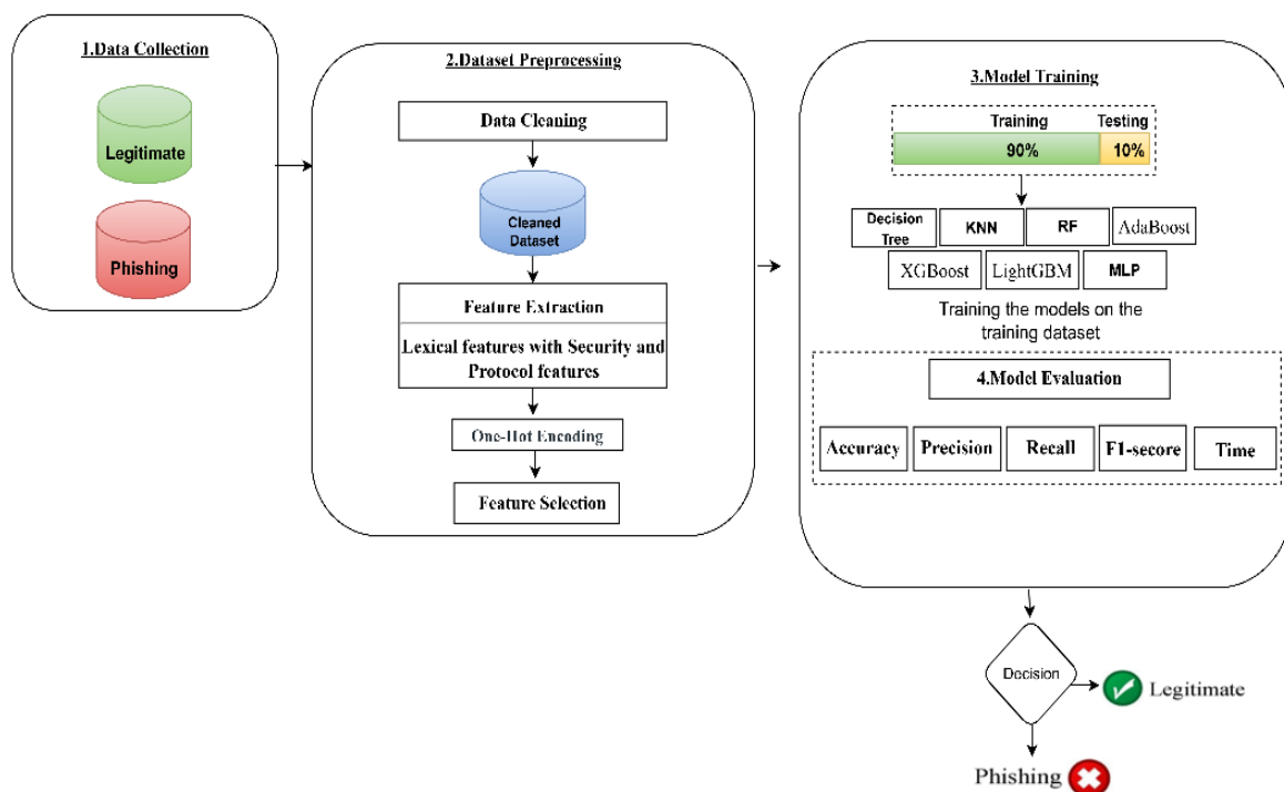
Figure 1. Overview of the proposed methodology (model development phase and output classification)
