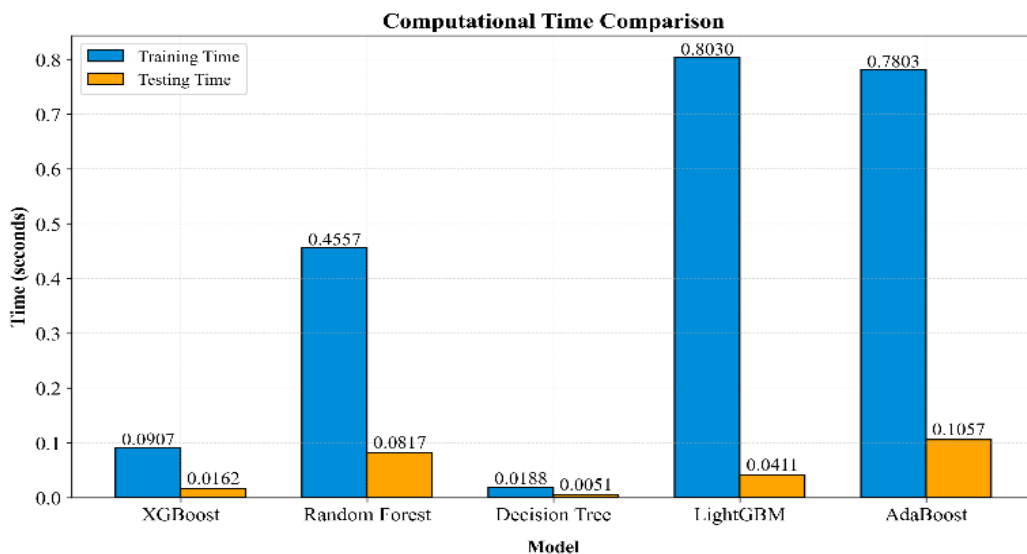
Figure 6. Comparison of training and testing computation times for ML models on 40 features
