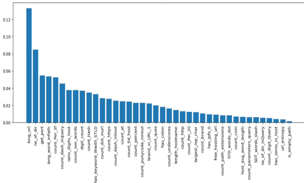
Figure 2. Gain-based feature importance obtained from the XGBoost model
