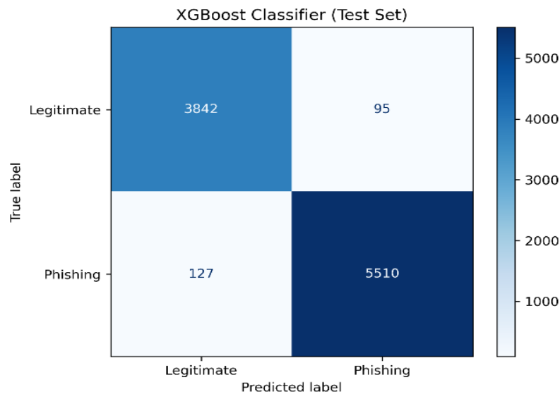
Figure 3. Confusion matrix of the XGBoost model
