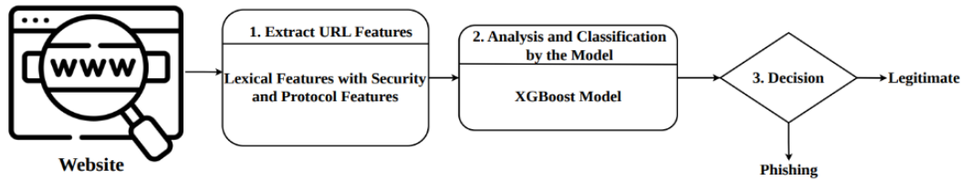
Figure 7. System architecture of the proposed model
