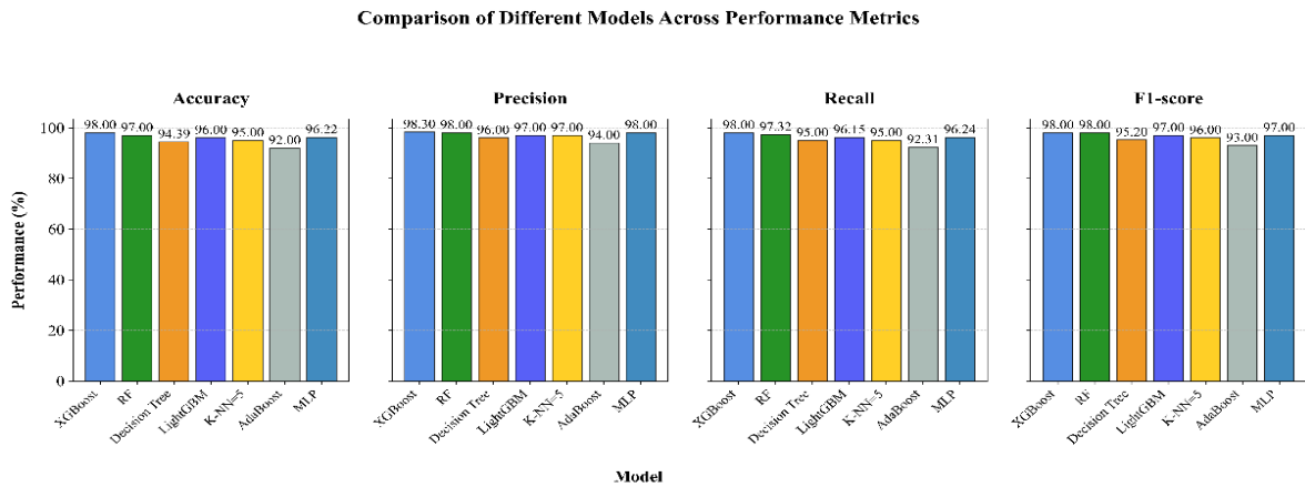
Figure 5. Performance of traditional ML models and MLP model trained on 40 features, with results calculated from the test set
