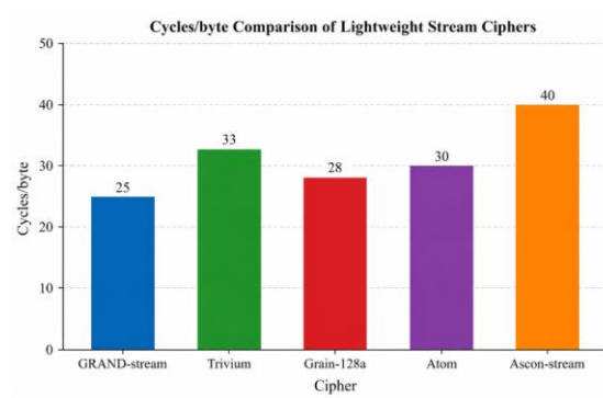
Figure 3. Comparison of cycles per byte for lightweight stream cipher algorithms
