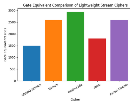
Figure 2. Gate equivalent comparison of lightweight stream ciphers
