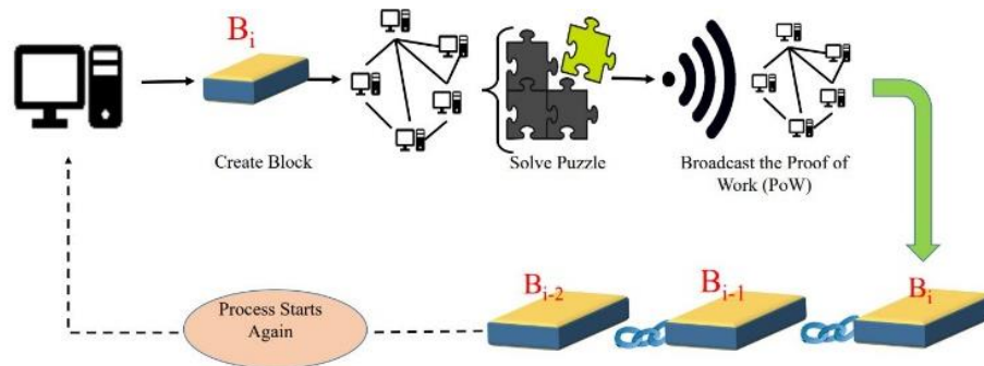
Figure 1. The mechanism of the consensus algorithm PoW [16]
