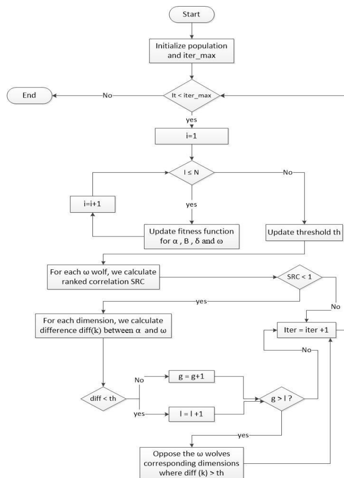
Figure 3. Flowchart of SO-GWO algorithm
