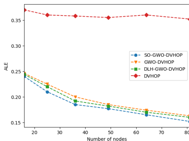
Figure 6. Variation of average location error of algorithms
