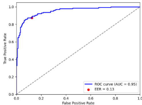
Figure 8. ROC curve
