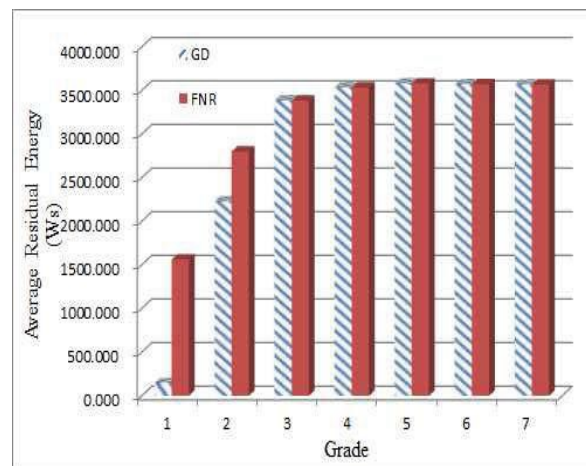
Figure 8. Average residual energy after 8000 events
