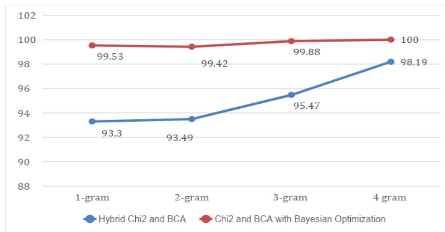
Figure 3. Graphic of Recall Performance
