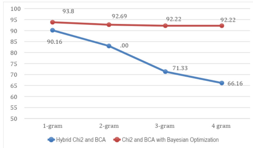
Figure 2. Graphic of Accuracy Performance
