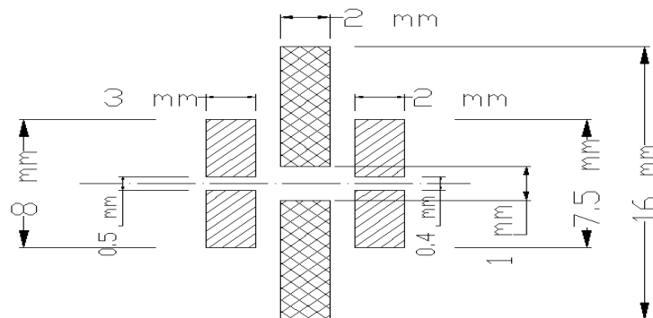
Figure 2. Two electrodes with the insulator
