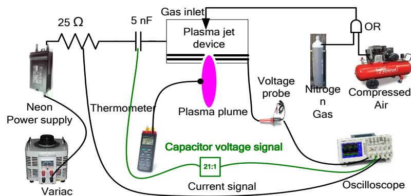
Figure 3. Experimental setup arrangement of the plasma jet device
