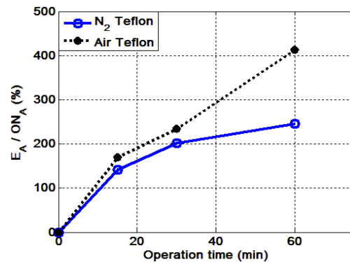
Figure 11. Ratio of (erosion area at different operation times / original area at t=0) % for the second group
