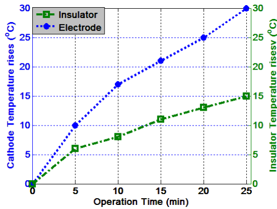
Figure 15. Temperature of cathode and insulator vs. operation time of Ceramic in ANPJ-II (Air)
