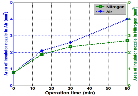
Figure 8. Area of insulator nozzle of second group vs. operation time of ANPJ-II
