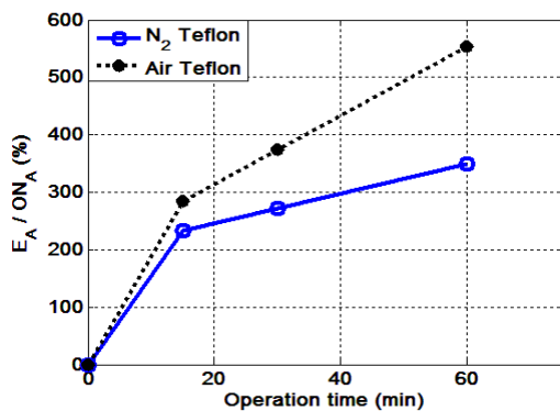
Figure 10. Ratio of (erosion area at different operation times / original area at t=0) % for the first group
