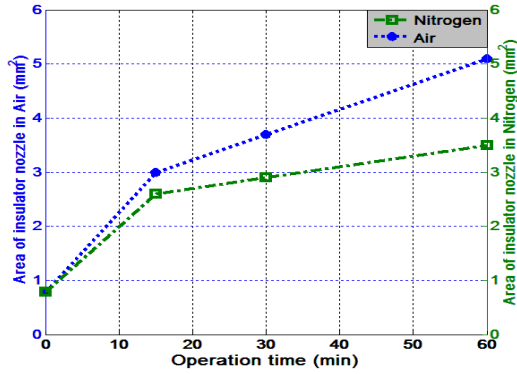
Figure 7. Area of insulator nozzle of first group vs. operation time of ANPJ-II
