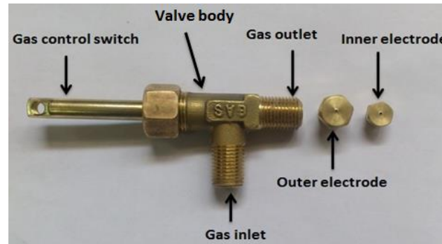
Figure 1. Gas valve and the two electrodes
