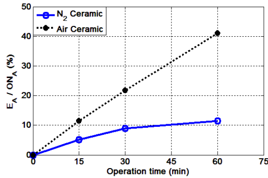
Figure 12. Ratio of (erosion area at different operation times / original area at t=0) % for the third group
