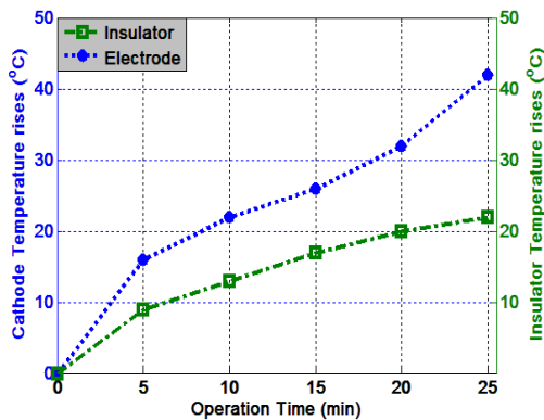
Figure 13. Temperature rises of cathode and insulator vs. operation time of Teflon in ANPJ-II (Air)
