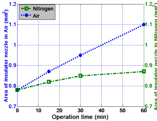
Figure 9. Area of insulator nozzle of third group vs. operation time of ANPJ-II
