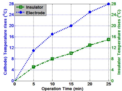
Figure 14. Temperature rises of cathode and insulator vs. operation time of Teflon in ANPJ-II (Nitrogen)
