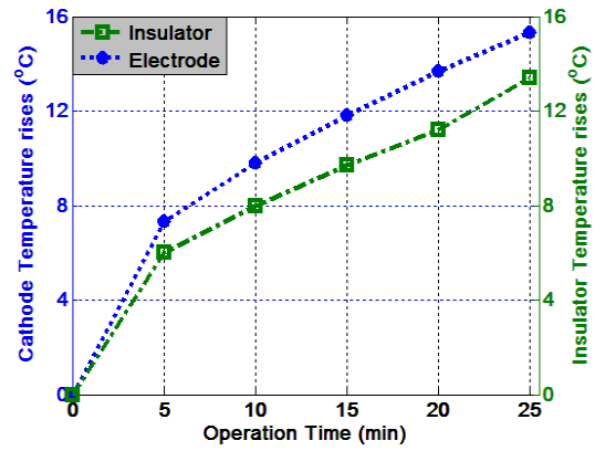
Figure 16. Temperature of cathode and insulator vs. operation time of Ceramic in ANPJ-II (Nitrogen)
