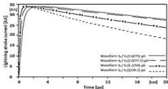
Figure 6. Lightning Source Wave Shape with Various Front Times
