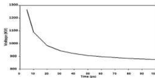
Figure 4. V-t curve of the 66 kV Insulator String
