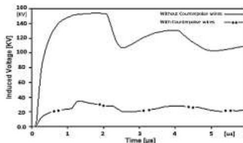
Figure 14. Footing Resistance Induced Voltage of Tower 1 Without and with using Counterpoise Wire
