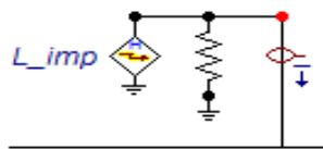
Figure 1. Simulation of Lightning Stroke Model
