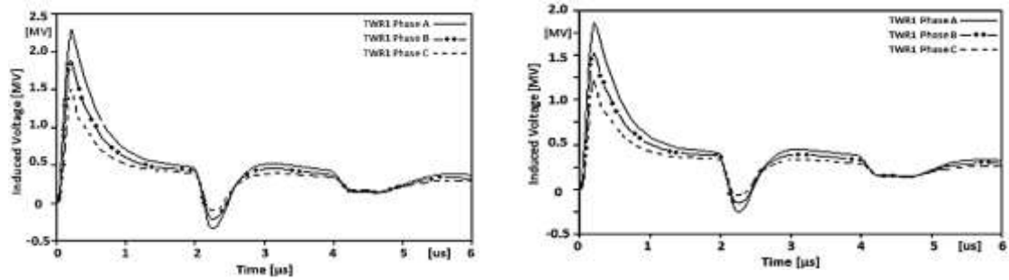
a) Induced Voltages of Phases A, B and C at Lightning Stroke Current Waveform 1.0/30.2 \mu s
