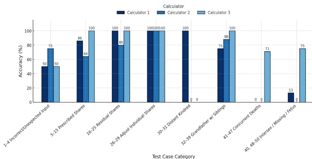
Figure 1. Accuracy of inheritance calculators by test case category
