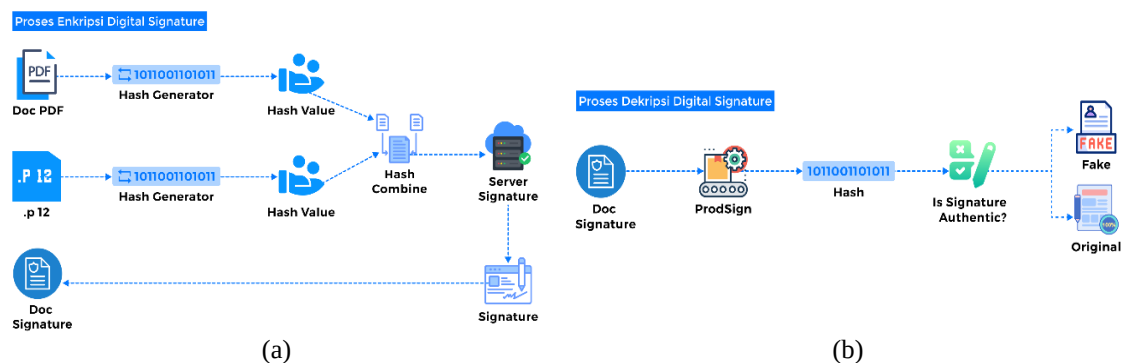
Figure 3. Illustration of the digital signature process (a) encryption/signing, where the document is processed using a hash value and private key to generate a digital signature, and (b) decryption/verification, where the document's authenticity is confirmed by comparing the regenerated hash with the original signature
