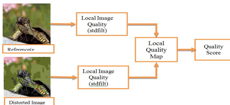
Figure 1. Overview of our LSDBIQ Model
