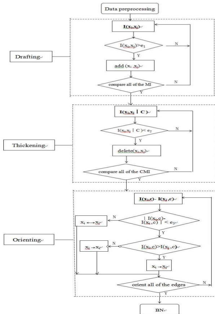
Figure 1. Bayesian Network Structure Learning
