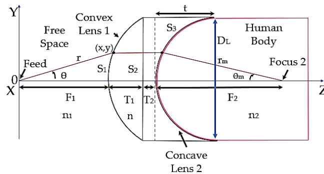
Figure 3. Focused lens structure for human body model
