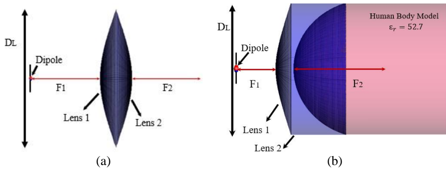
Figure 7. Simulation models for investigating the focal spot size using focused lens; (a) focused lens in the free space and (b) focused lens for the human body model
