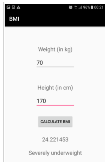
Figure 6. BMI interface
