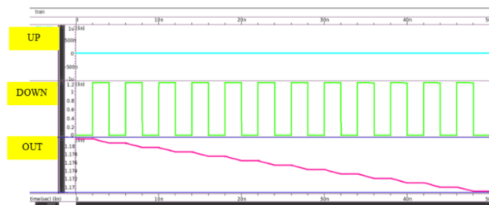
Figure 13. Output waveform in discharging condition
