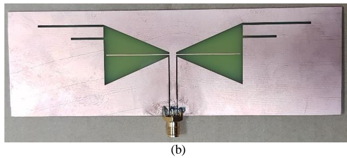
Figure 1. Antenna (a) geometry (b) fabricated antenna in state one
