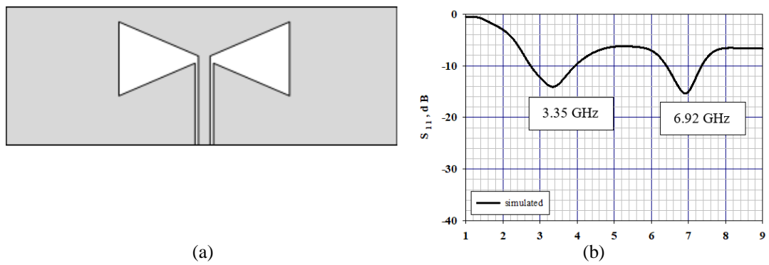
Figure 2. Reference slotted bowtie antenna (a) geometry (b) S_{11}
