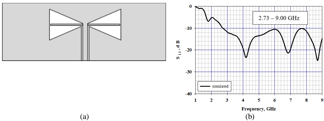
Figure 3. Reference slotted bowtie antenna with rectangular box (a) geometry (b) S_{11}
