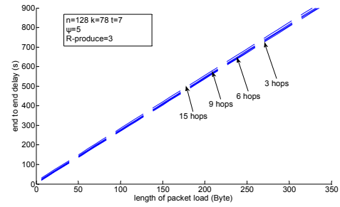
Figure 10. Delay vs Payload for Different n_{hop}
