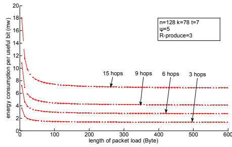
Figure 9 Energy vs Payload for Different n_{hop}
