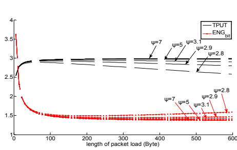
Figure 7. Throughput &amp; Energy vs Payload
