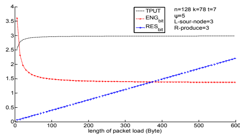
Figure 6. Objective Functions vs Payload
