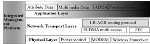
Figure 1. Micro-ANP Protocol Architecture
