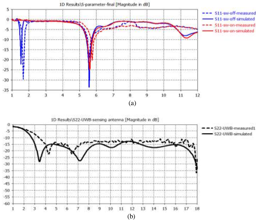
Figure 4. (a) The simulated and measured S-parameter versus frequency of (a) the communicating antenna (b) the UWB sensing antenna
