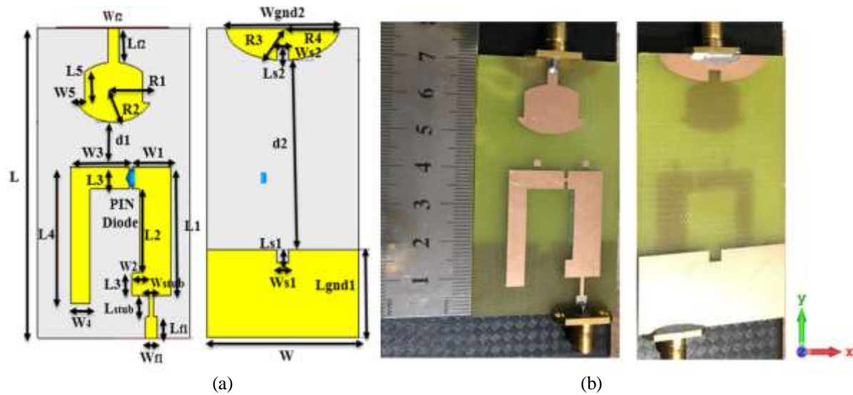
Figure 2. The proposed multi-band cognitive radio antenna, (a) Front side, (b) Backside
