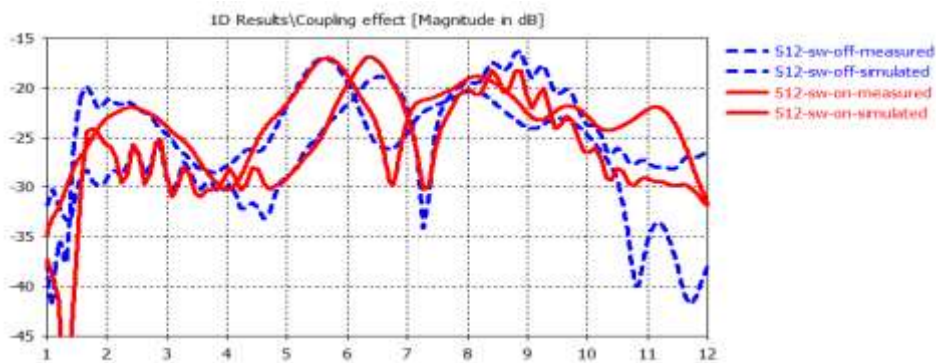
Figure 5. The simulated and measured (S12) parameter (Coupling effect) between the two antennas versus frequency
