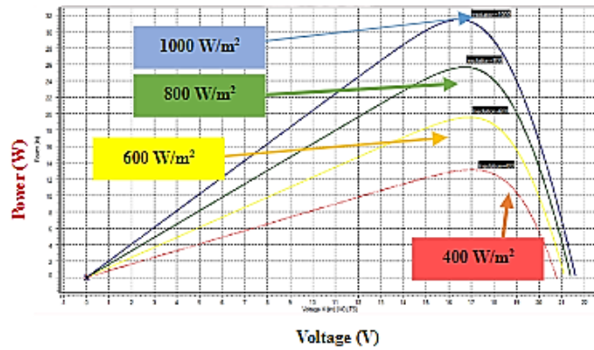
Figure 1. Power-voltage P-V characteristic curve of the solar panel under varying irradiances (400, 600, 800, and 1000 W/m 2 ) at 250C
