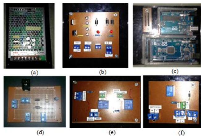
Figure 5. Devices of the Project: (a) Switched Mode Power Supply, (b) Regulator Circuit, (c) Arduino, (d) Buck Boost Converter Circuit, (e) Source Switching Circuit and (f) Diversion Load Controller Circuit
