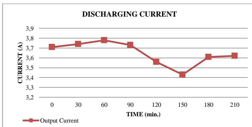
Figure 12. Current delivered to the two 30-watt load
