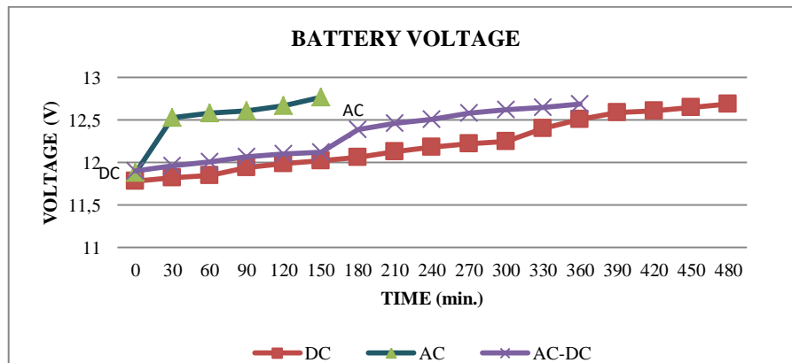
Figure 9. Battery voltage while charging using the different sources
