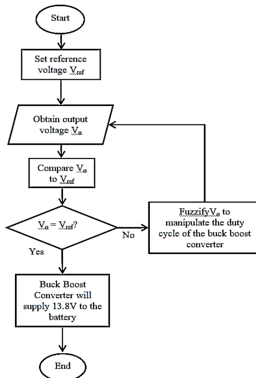
Figure 6. Fuzzy Control input flowchart
