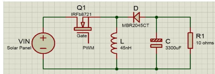
Figure 2. Buck Boost Converter Inverting Topology [15-17]
