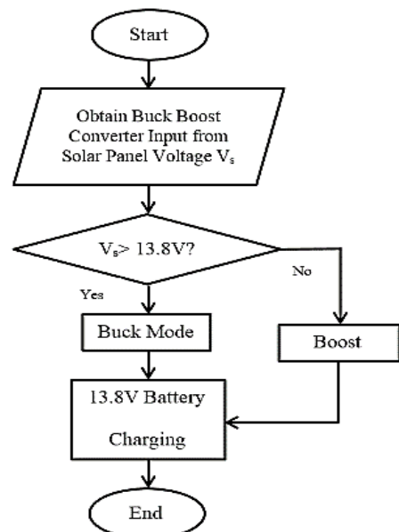
Figure 3. Buck-Boost Converter Input Flowchart
