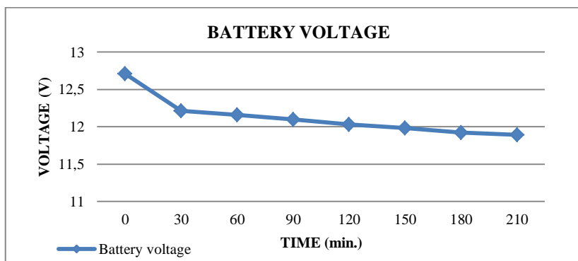
Figure 11. Battery voltage while discharging
