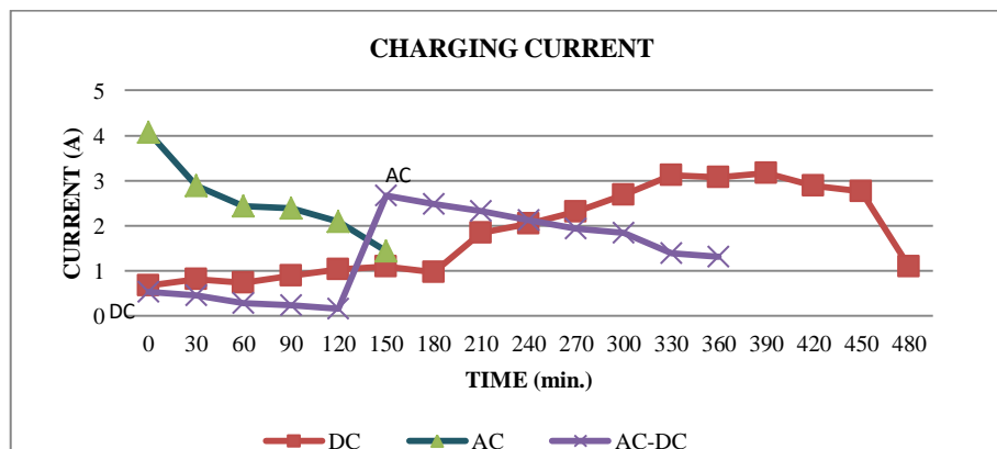
Figure 10. Charging current of different sources
