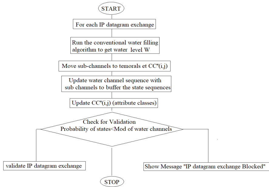
Figure 2. Flowchart of the proposed algorithm describing the workflow process
