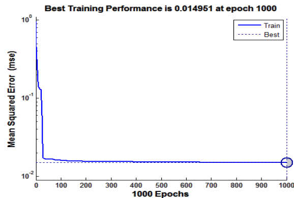
Figure 4. The performance analysis of the cascaded neural network during the classification phase
