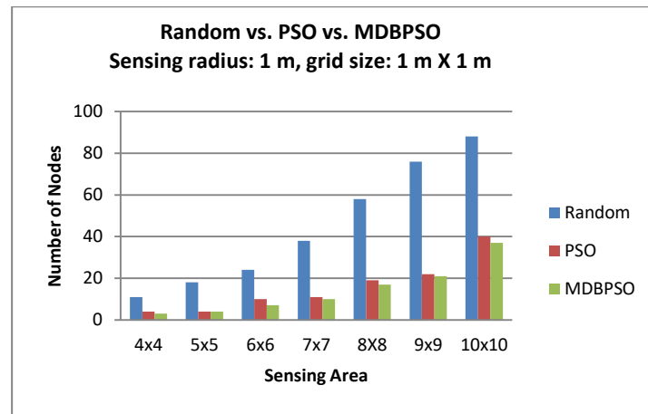
Figure 6. Comparison of Random PSO & MDBPSO for Sensing Area vs Number of nodes for Square grid area
