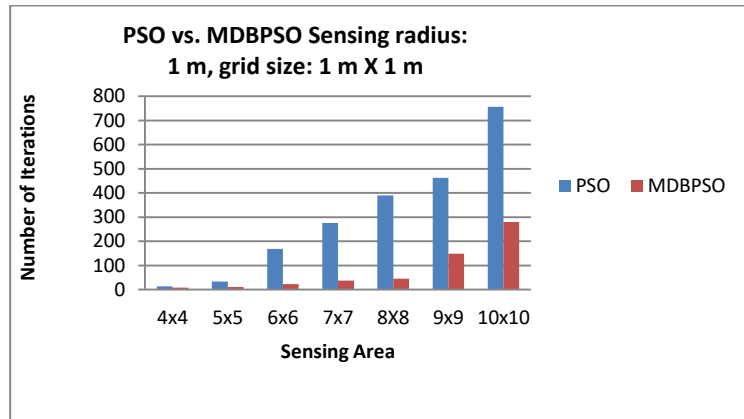
Figure 4. Comparison of PSO & MDBPSO for Sensing Area vs Number of iterations
