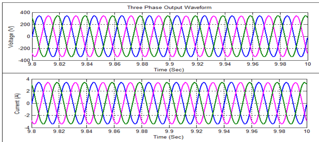
Figure 6. Stator Voltage and Current Waveform
