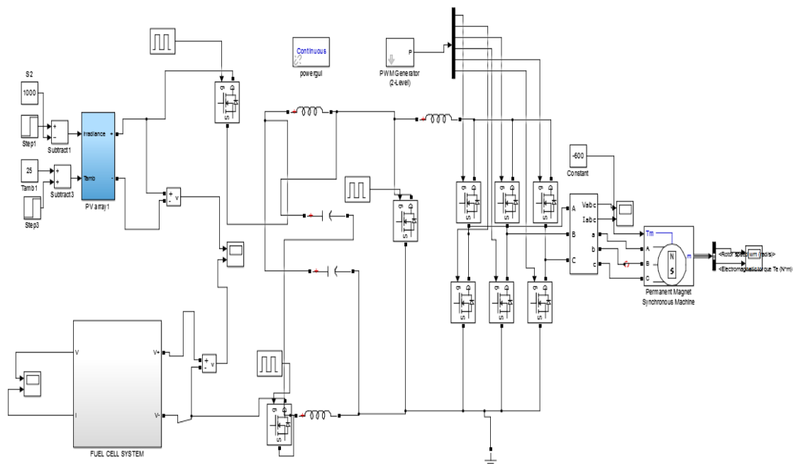
Figure 3. Overall Proposed Simulation Circuit Method
