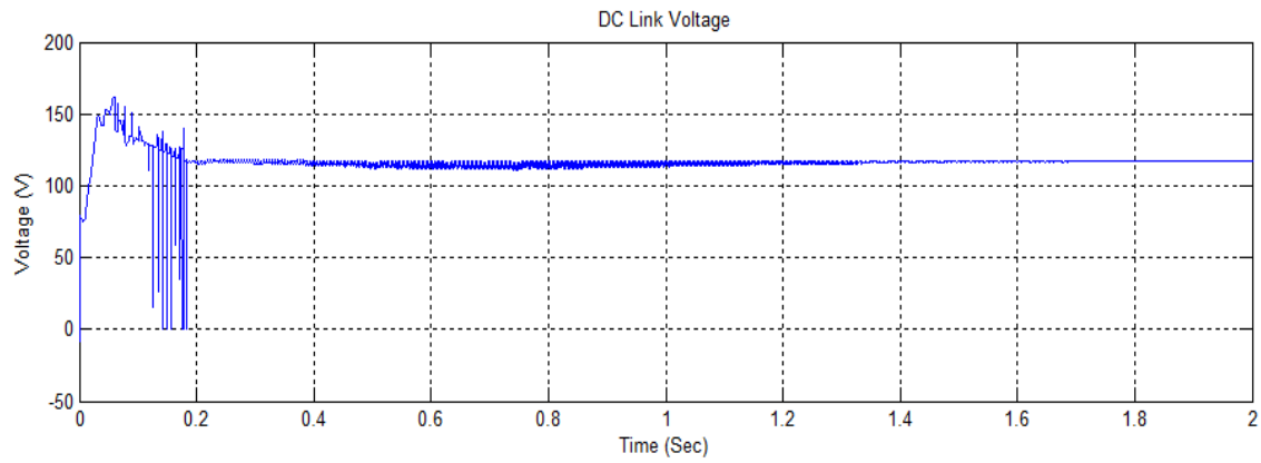
Figure 5. DC Link Voltage
