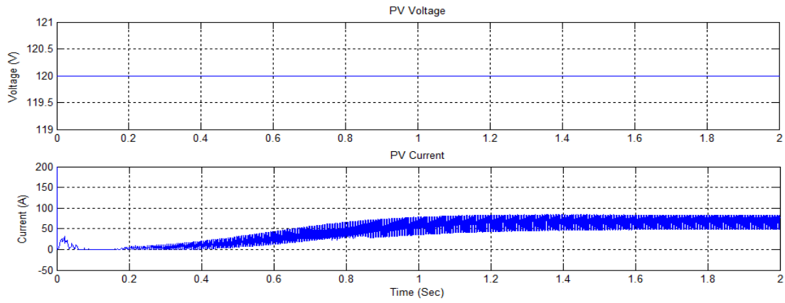
Figure 4. PV Voltage and Current Waveform
